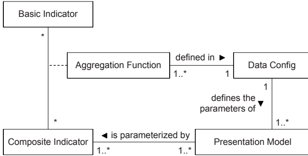
Figure 4. The relation between presentation model and data config
